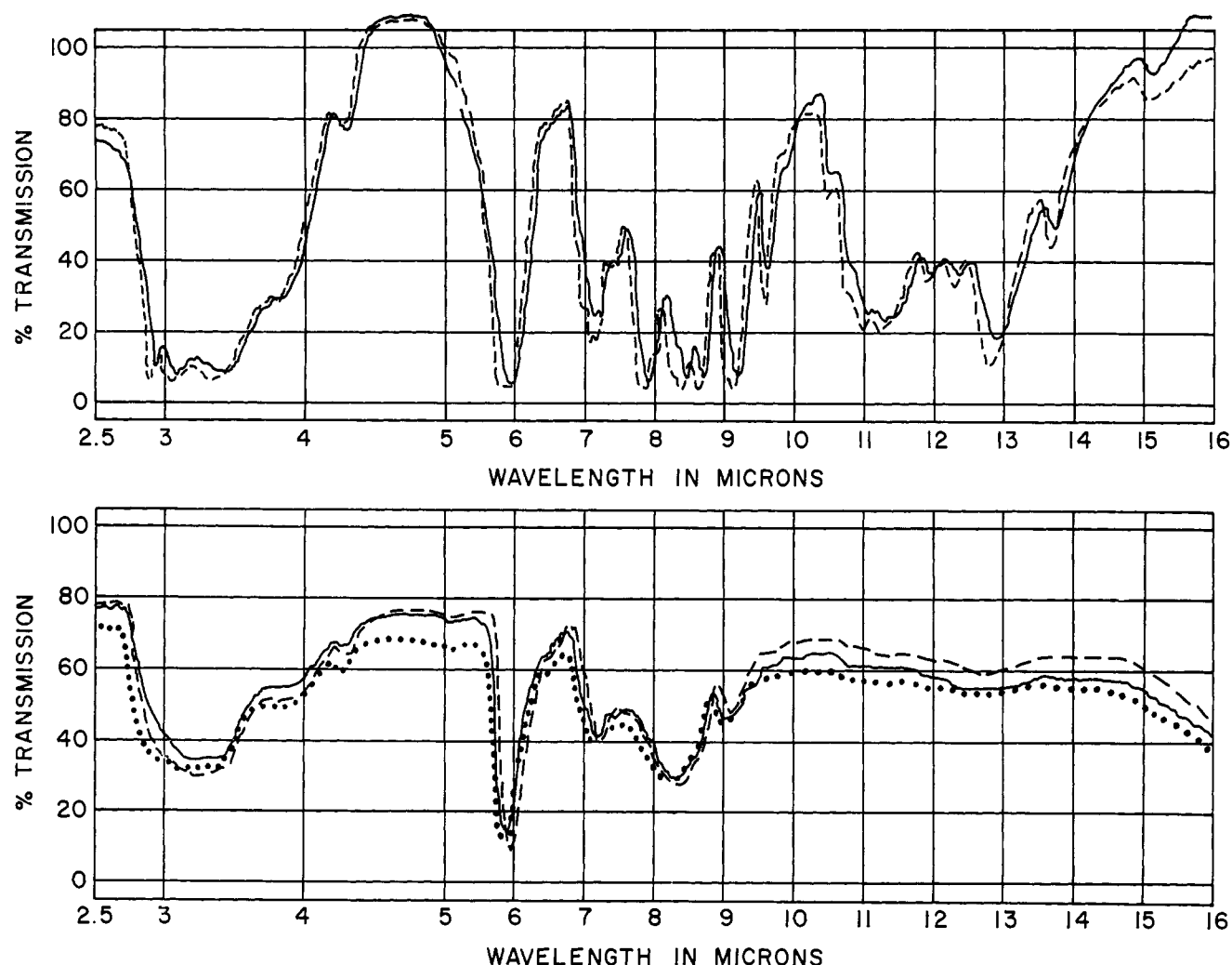
FIGURE 4: Infrared spectra of natural and synthetic threo -homoisocitric acid. Top chart: samples were run in KBr pellets on a Beckman IR-8 spectrophotometer. (---) Crystalline, racemic threo -homoisocitric acid prepared by ozonolysis (offset 0.1 \mu for comparison); (—) crystalline racemic threo -homoisocitric acid prepared according to the method of Yamashita (1958). Bottom chart: samples were run neat on NaCl plates. (····) Amorphous (—)- threo -homoisocitric acid prepared by ozonolysis; (—) amorphous natural homoisocitric acid isolated from mutant of S. cerevisiae ; (---) amorphous, racemic threo -homoisocitric acid prepared according to Yamashita (1958).
