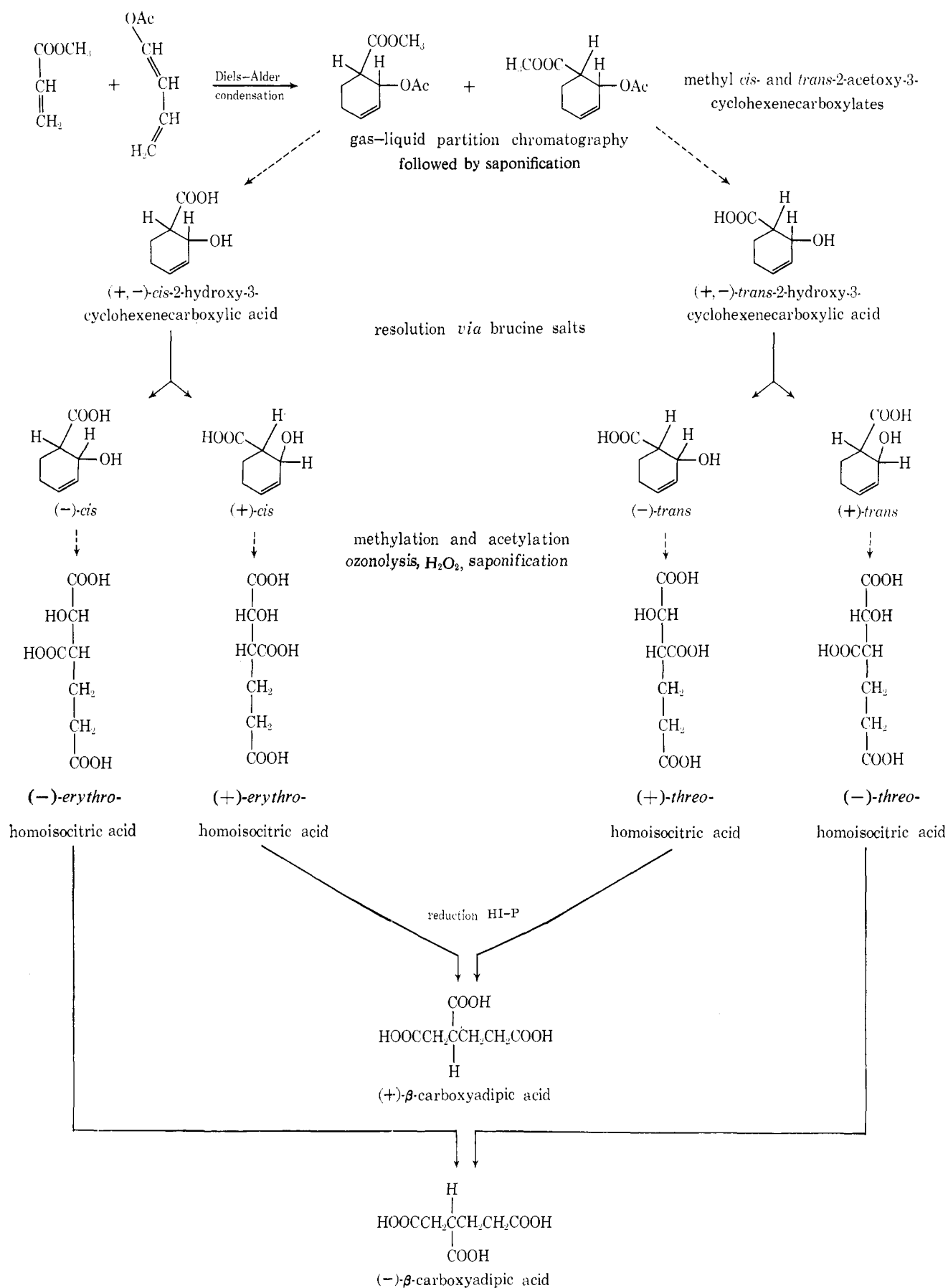
FIGURE 2: Synthesis and proof of absolute configuration of the optical isomers of homoisocitric acid.
